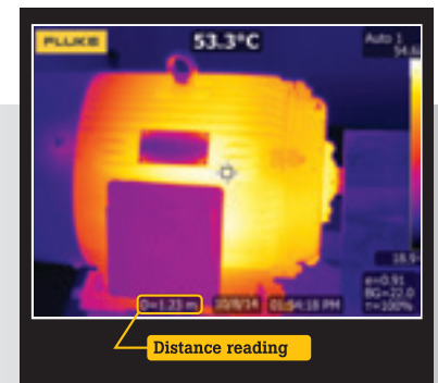
LaserSharp® Auto Focus uses a built in laser distance meter that calculates and displays the distance to your designated target with pinpoint accuracy.
