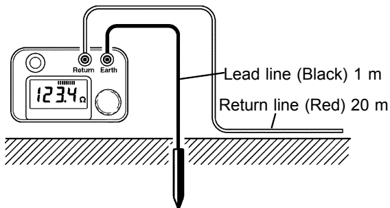
Figure 3. Connection Diagram
